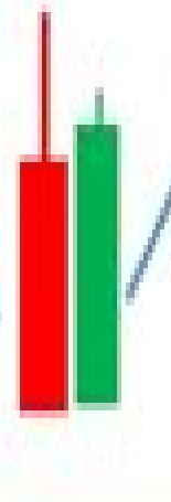
Bullish Tweezers
