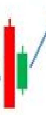
Bullish Harami
