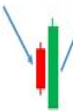
Bullish Engulfing
