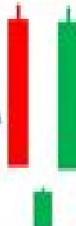
Morning Star
