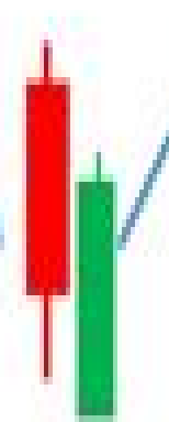
Piercing Pattern
