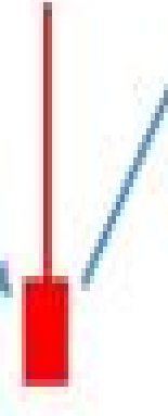
Inverted Hammer
