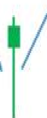
Hammer
