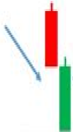
Bullish Counterattack
