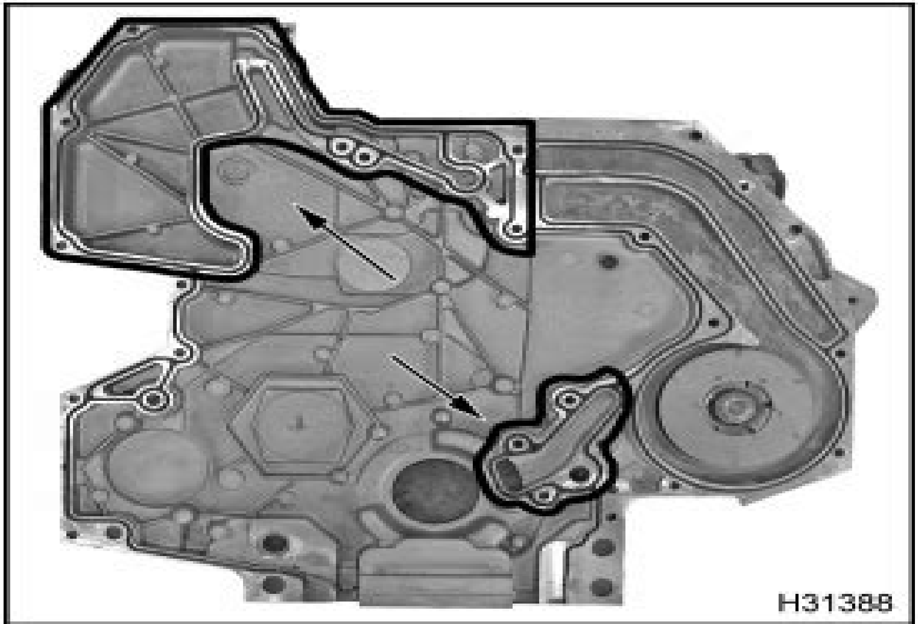
Figure 158 Front cover oil pressure leak locations
