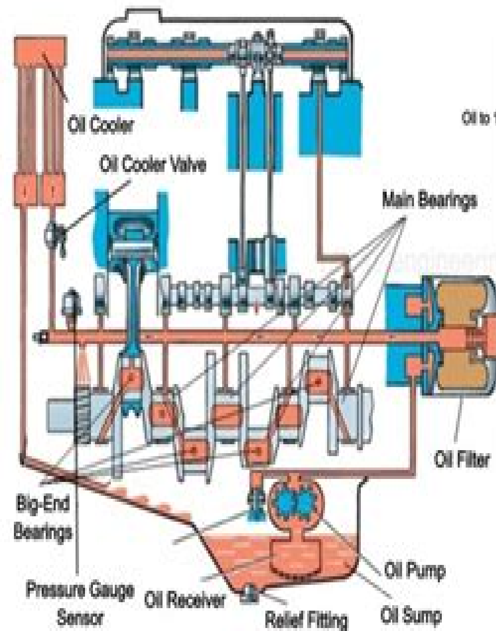
Types of Lubrication System
