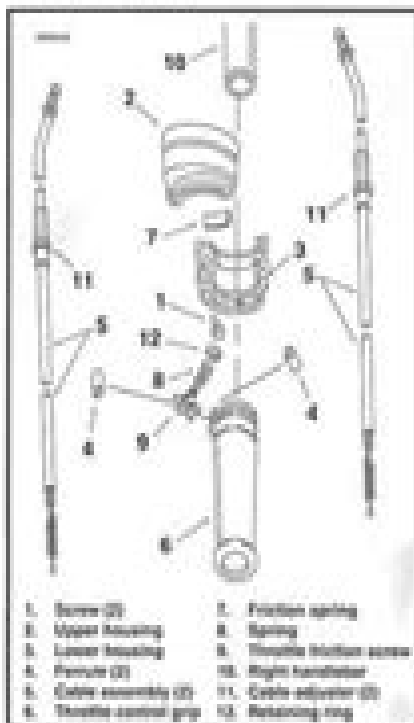
Figure 2-78. Throttle Control - Right Handlebar
