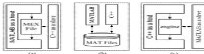
Figure 1. Algorithm development environments by using: MATLAB as a host and C++ MEX functions (a); C++ as a host which executes MATLAB's functions and exchange data (b); MATLAB and C++ separately with storing intermediate results in MAT file for re-use or result comparison, cf. Ref [3].
