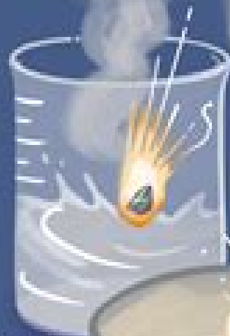
THERMITE REACTION
