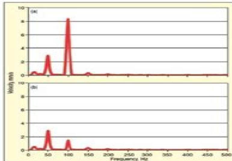
Figure 2. Vibration spectrum generator drive and bearing: (a) with load dispatch; and (b) immediately after power removal.
