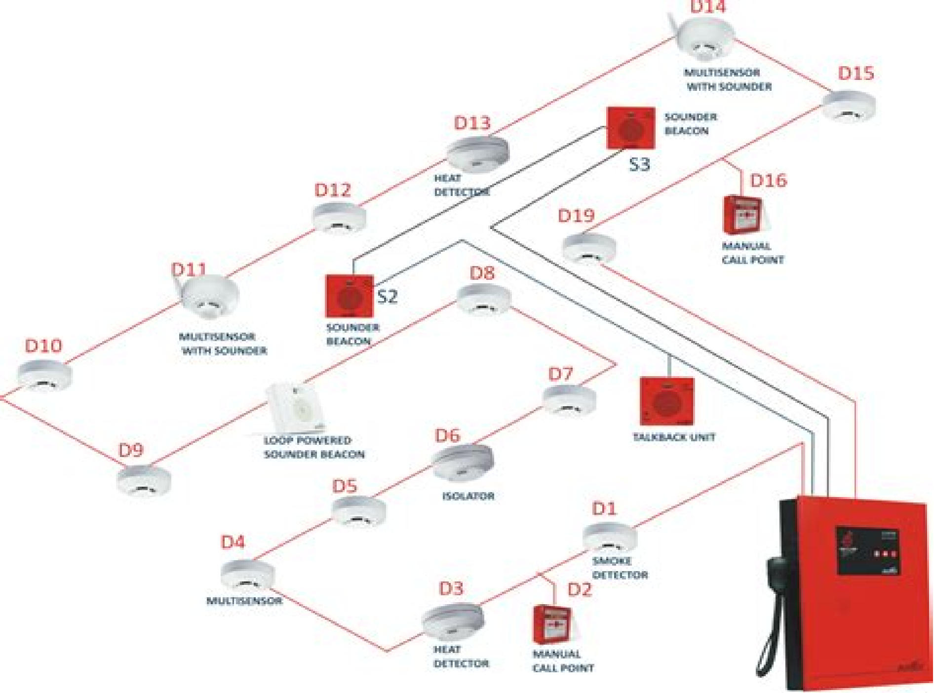
CONTROL PANEL
