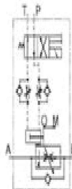
Pilot Operated Flow Control and Check Valve
