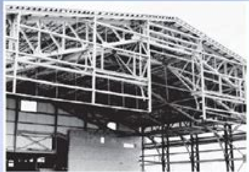
Figure 5-5(a) Type II or noncombustible construction
