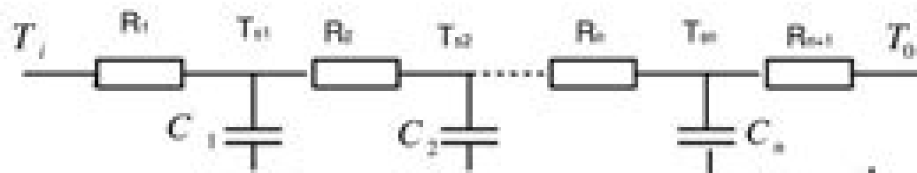
(c) n-th order lumped model
