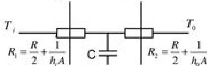
(b) 2R1C lumped model
