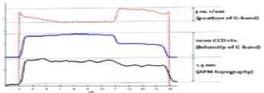
Fig. 2: Variations in G-band position and G-band intensity in comparison with the height profile of the AFM topography image.
