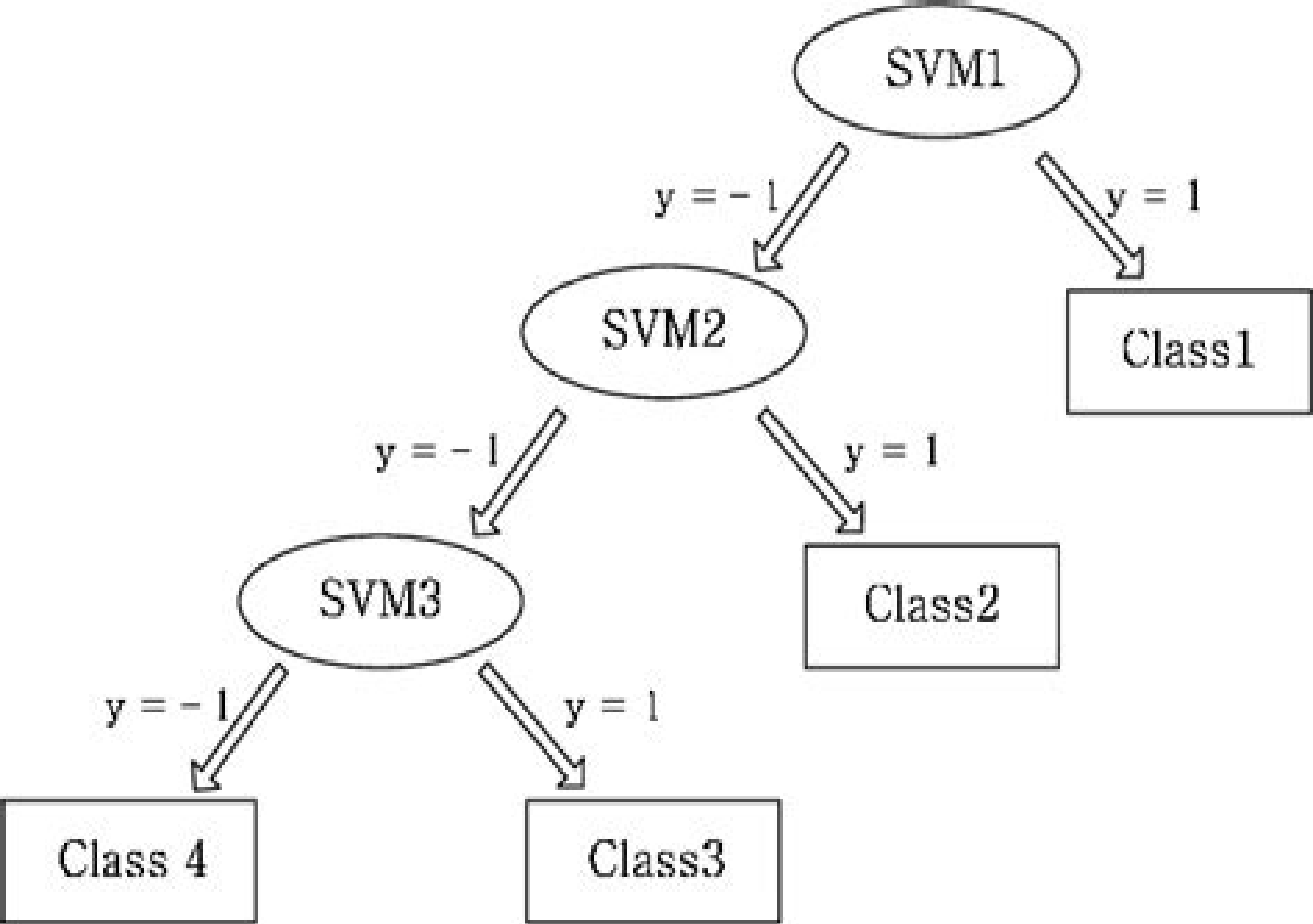
Fig. 2 Multi-class system classified by the HCM
