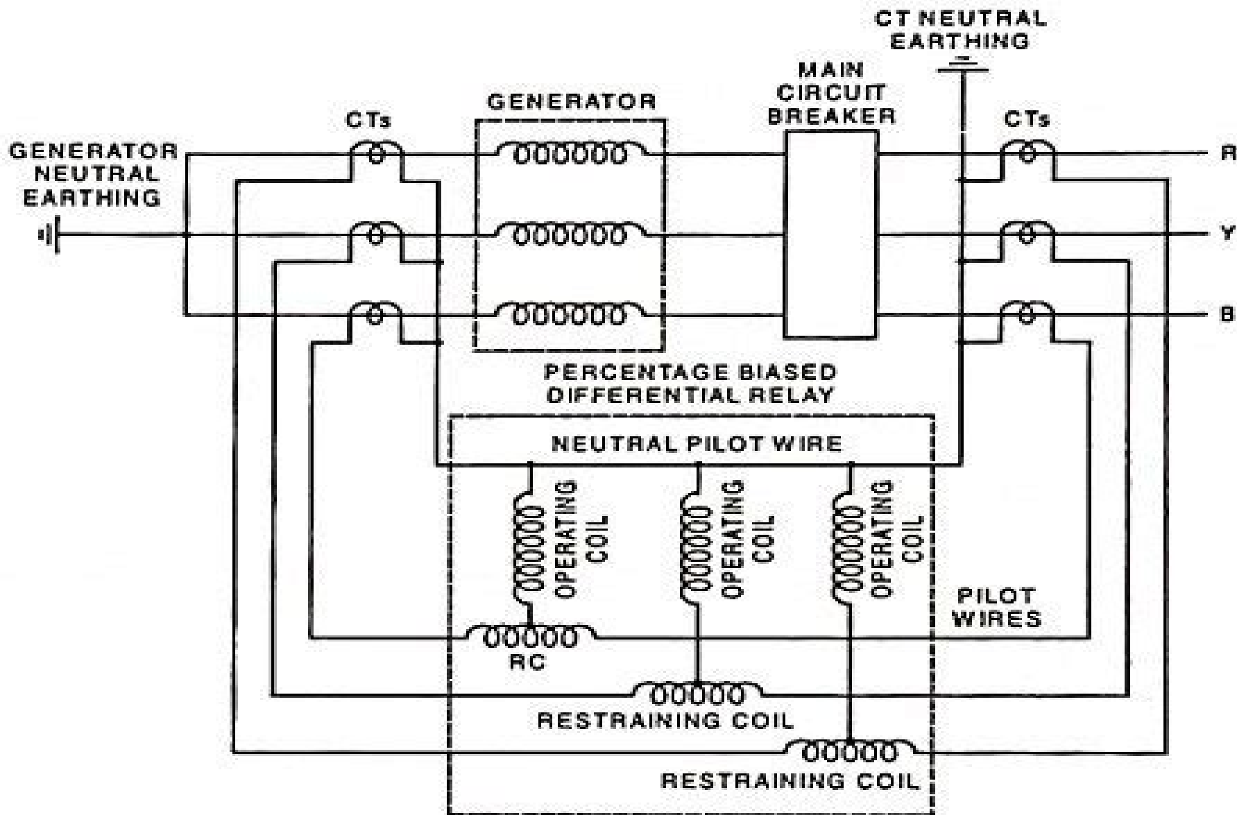
Fig. 11.4. Schematic Diagram For Percentage Differential Relay Protection of a Star-Connected Generator
