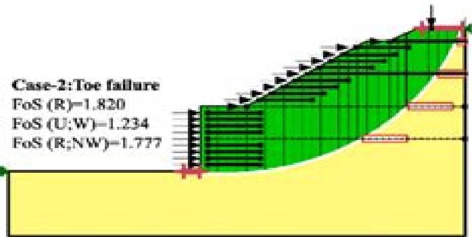
Case-2: Berm failure FoS (R)=2.002 FoS (U;W)=1.116 FoS (R;NW)=1.777
