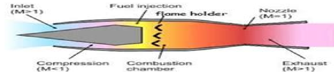
Figure 4.5 ramjet
