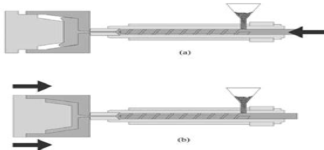
Figure 1.18 Injection-compression moulding
