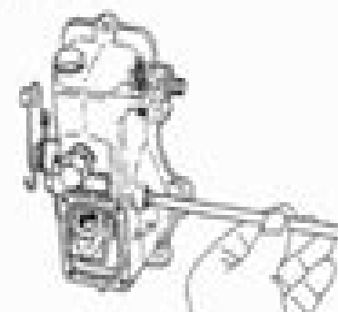
(9) After you remove the O-ring, lightly tap the end of the shaft that you removed the O-ring from, and remove the governor lever shaft. Then remove the governor shaft assembly and wash it.
