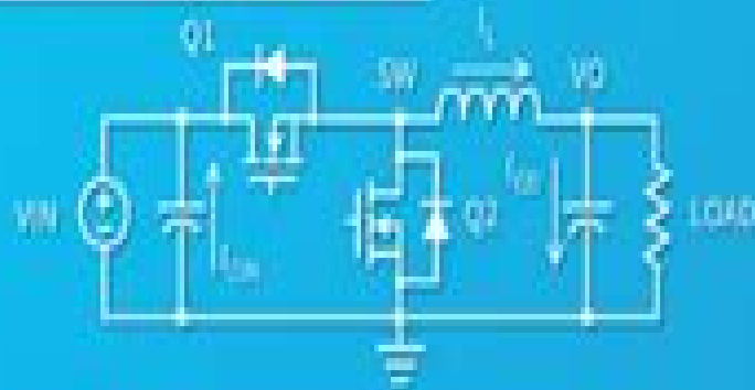
Inductor Charging Mode
