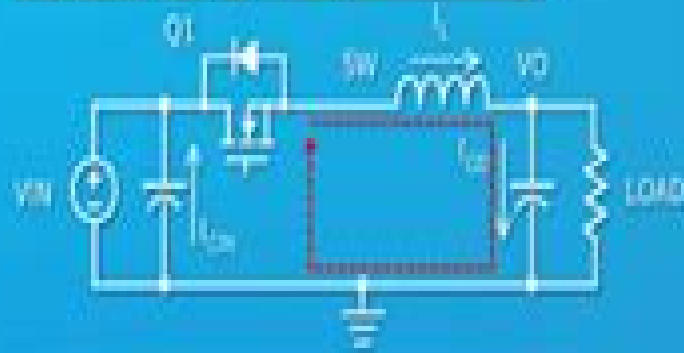
Inductor Discharging Mode
