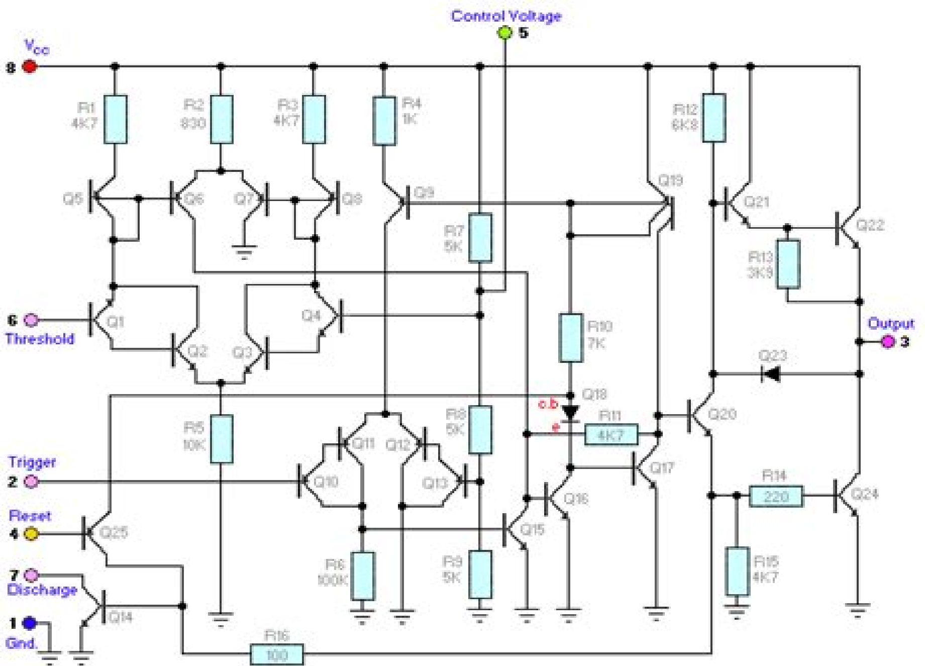
555 Schematic
