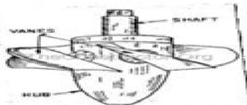
Fig.1.1 Kaplan Turbine Hub with Blades
