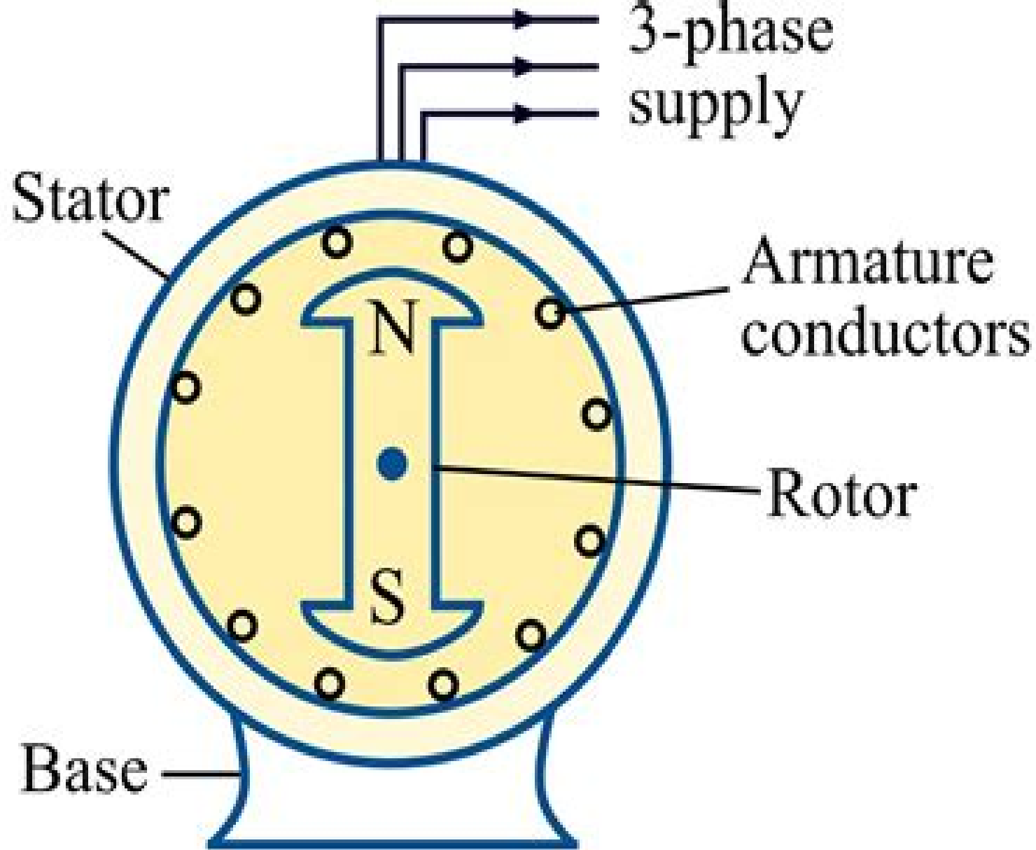
Figure 1 - Synchronous Generator
