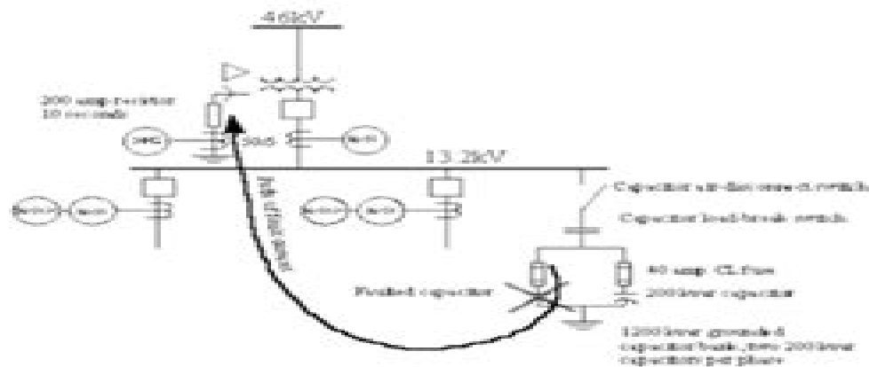
Figure 1 - Typical industrial facility showing ground fault protection system, failed capacitor, and fault current path for a failed capacitor.
