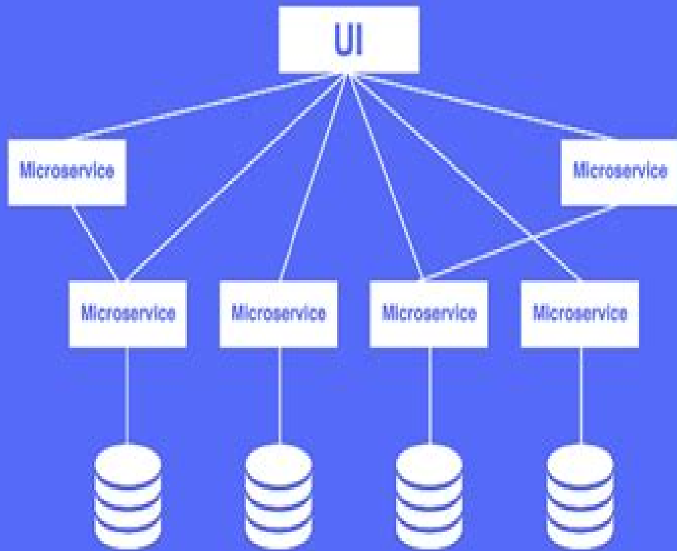
Microservices Architecture
