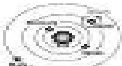
HELIOCENTRIC
