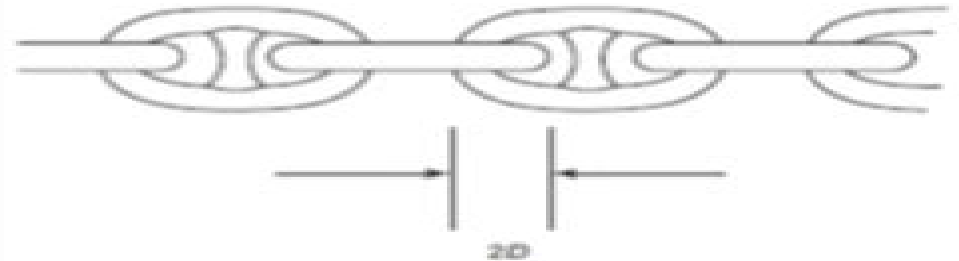
c) Two diameter measurements (Offshore Inspection Method)
