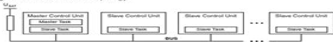
Figure 1. LIN Network Topology
