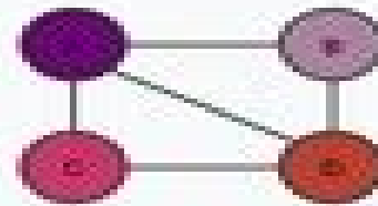
Undirected Graph
