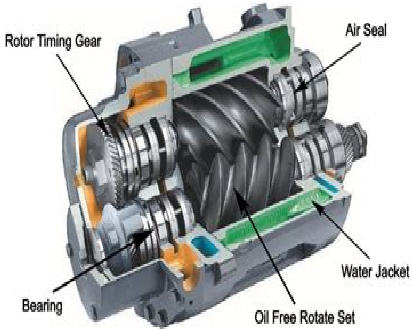
Rotary Screw Compressor
