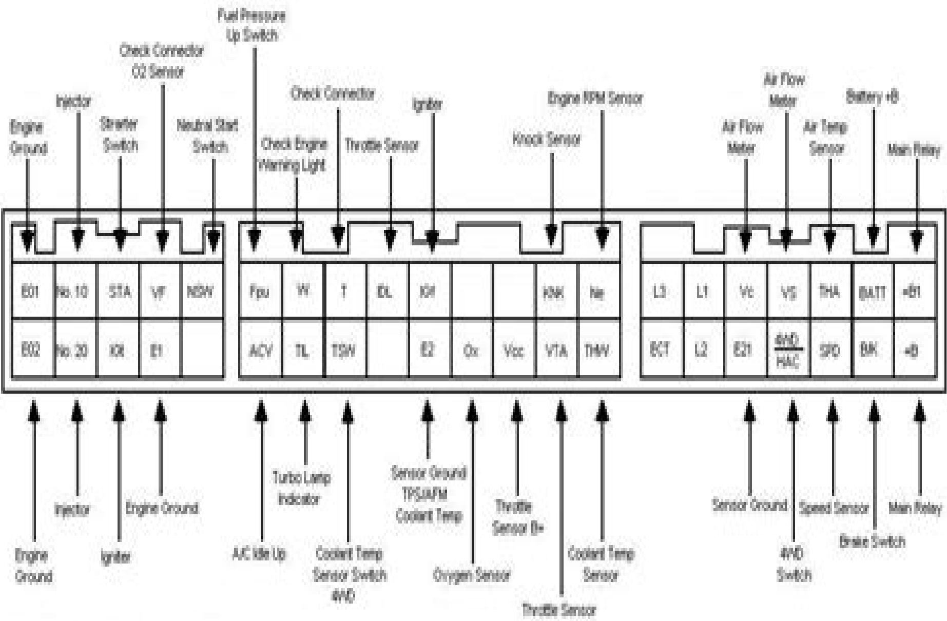
ECU Pinouts for 88 Toyota Truck w/2RTE
