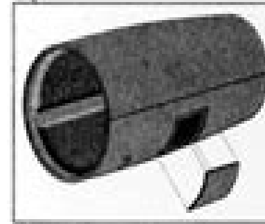
NACELLE • Carbon Fiber/Epoxy • Aluminum Honeycomb
