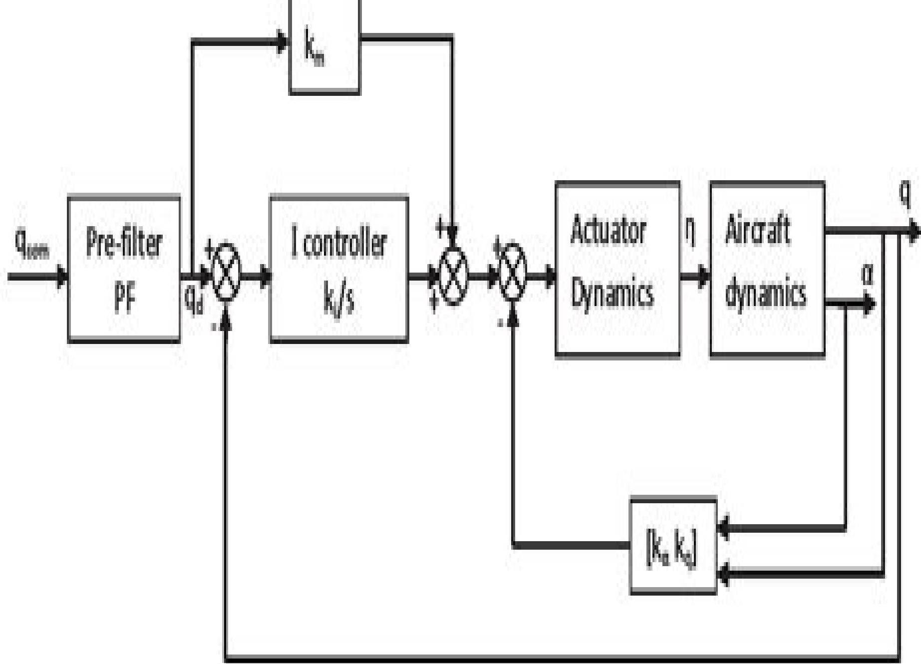
rate command/attitude hold flight control system
